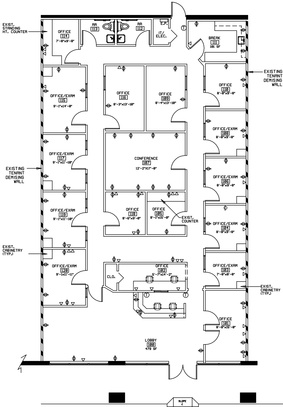
1 FLOOR PLAN SUITE: C SQUARE FOOTAGE: 3,300 RSF
